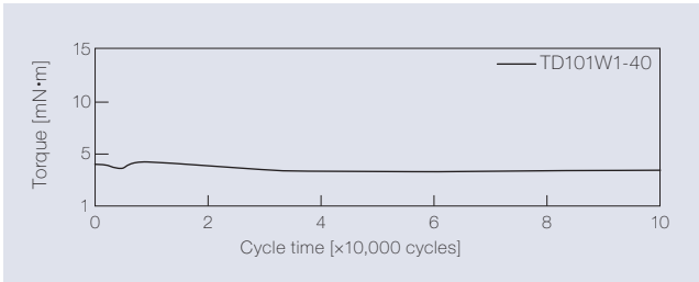
Measurement of torque at a rotation speed of 30 min -1
