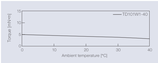
The torque achieved during rotation at 30 min -1 in the designated ambient temperature is shown.
